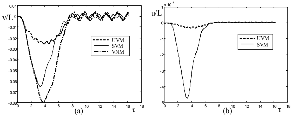
Figure 10. Non-dimensional a) transversal deflections and b) longitudinal deflections of the tip point found by different models for \omega_0^*=3.51 , T^*=8.1 .
