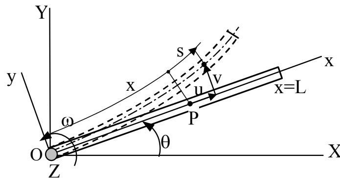
Figure 1. Rotating beam in its deformed position.
