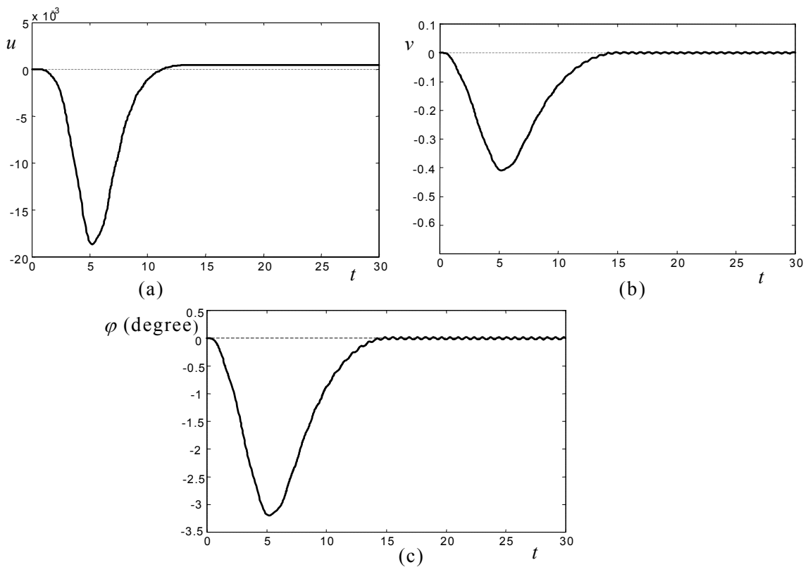
Figure 14. Longitudinal deflections (a), transversal deflections (b), and slopes (c) of the tip point found from the SV \varphi M (based on the input data given in [14]).
